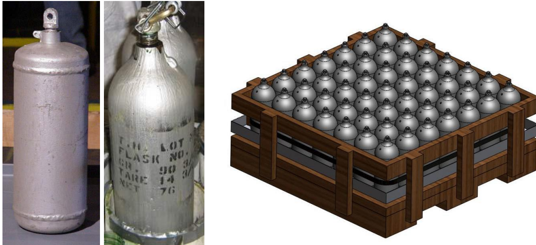
Picture 16. Examples mercury packaging - standard 3 litre elemental mercury flasks individually and packed in a 49 x 3 litre crate will built in spill tray. Source: US DoE (2009)
