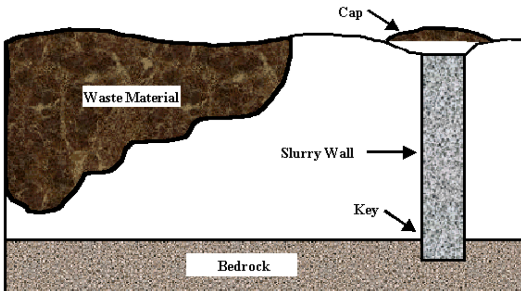
Picture 9: Section showing capped slurry wall isolation
