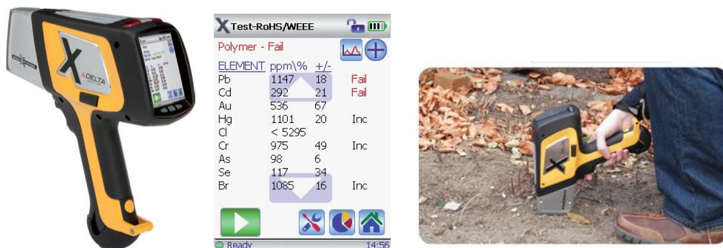
Picture 2: The Olympus Delta portable X-Ray Fluorescence Analyser with screen shot example of digital screen readout for metals in polymer. Source: www.innovx.com
