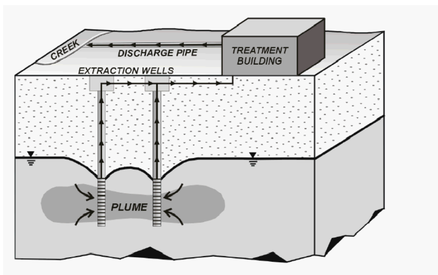
Picture 13: Pump and treat principles. Dept. of Geosciences Texas A&M University
