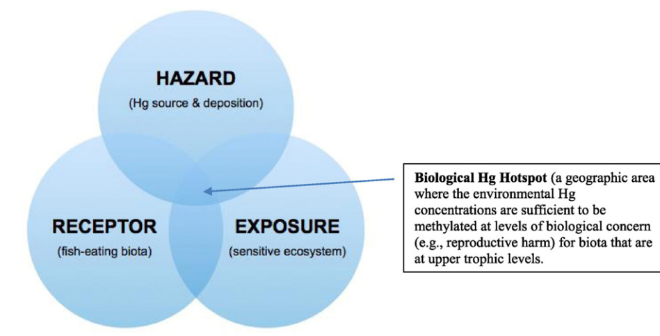
Fig. 4. A Venn diagram illustrating the critical relationships among three components of the Hg issue: (1) Hazard (magnitude of Hg source and its transport and fate); (2) Exposure (sensitivity of ecosystem to methylating Hg); and (3) Receptor (trophic level of bioindicator).
